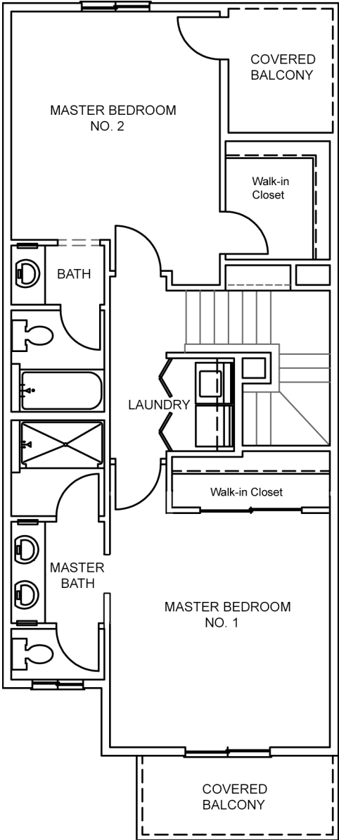
2nd Floor
